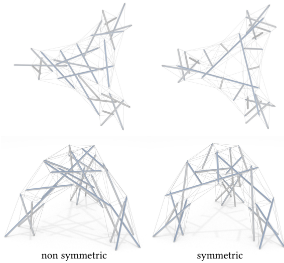
Fig. 7. Stable structures obtained with and without rotational symmetry constraint during the initialization (above: top view; below: side view).
