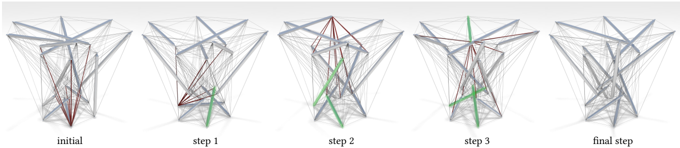
Fig. 8. Exploring the space of possible connectivities that leads to a stable configuration after 11 steps. For each step, the set c of additional hard constraints is shown in Red, while the green strut is the one inserted in the step m + 1 to accommodate the constraint c_m defined on a previous step.
