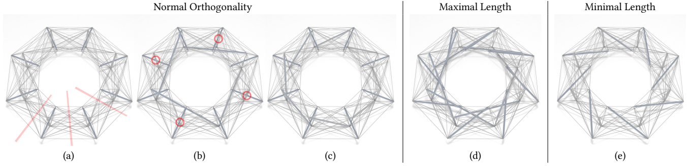
Fig. 6. Examples of Connectivity Finding results, for three different choices of likelihood criterion, as reported on top. (a) only Connectivity constraints are enforced; (b) Cutting-Planes constraints are added—three planes violating this constraints are shown in (a); (c-d-e) Minimal Strut-to-Strut Distance constraint added—violations of this constraint are circled in (b).
