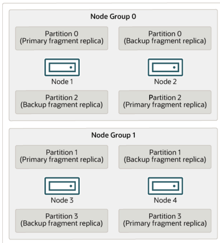
Figure 2.2 NDB Cluster with Two Node Groups
