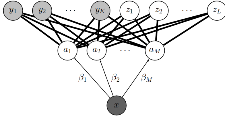
(a) Direct Attribute Prediction (DAP)
