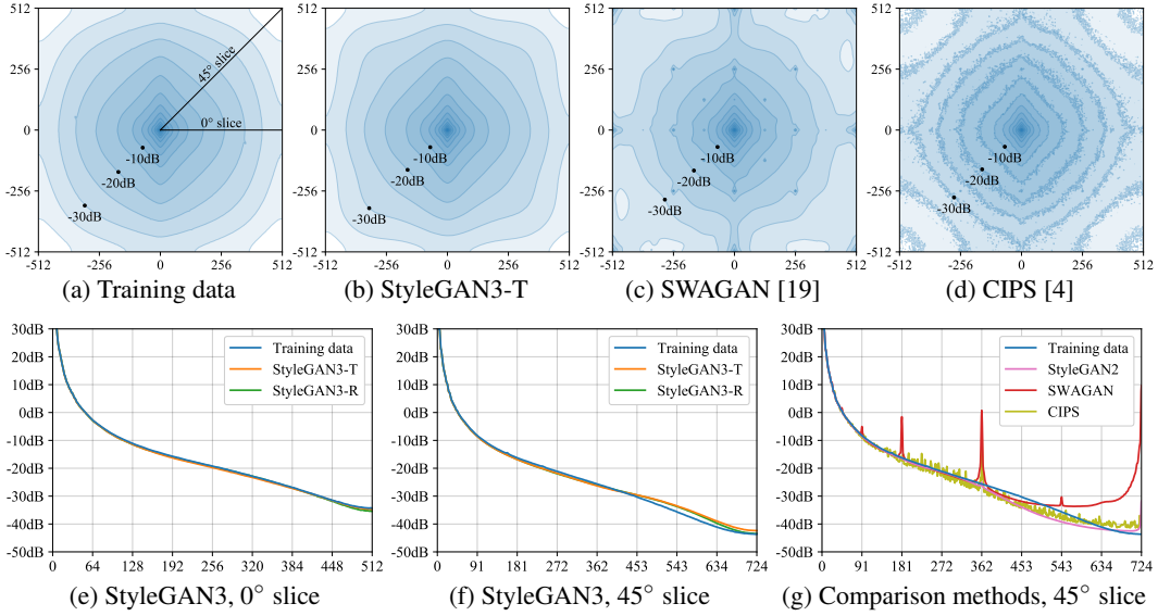
Figure 13: Top: Average 2D power spectrum of the training images in FFHQ at 1024x1024 resolution, along with the corresponding spectra of random images generated using StyleGAN3-T, SWAGAN [19], and CIPS [4]. Each plot represents the average power over 70k images, computed as follows. From each image, we subtract the training dataset mean, after which we divide it by the training dataset standard deviation. Note that these normalizing quantities represent the entire dataset reduced to two scalars, and do not vary by color channel or pixel coordinate. The image is then multiplied with a separable Kaiser window with \beta = 8 , and its power spectrum is computed as the absolute values of the FFT raised to the second power. This processing is applied to each color channel separately and the result is averaged over them. These spectra are then averaged over all the images in the dataset. The result is plotted on the decibel scale. Bottom: One-dimensional slices of the power spectra at 0° and 45° angles.
