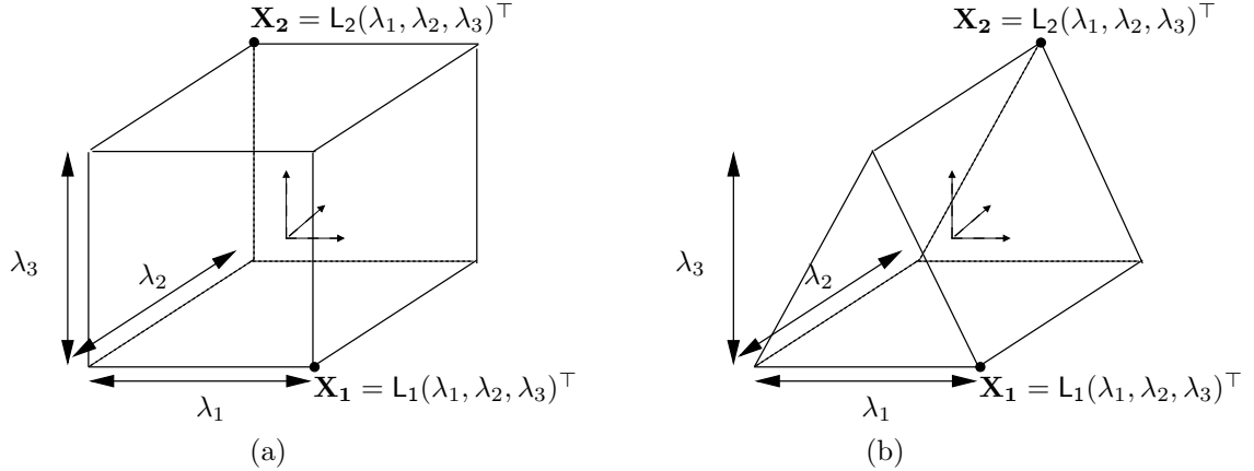
Figure 1.10: Examples of linearly parameterized models [Debevec et al., 1996; Jelinek and Taylor, 2000]. (a) Cube; points \mathbf{X}_1 and \mathbf{X}_2 are parameterized by, respectively, matrices \mathbf{L}_1 = \text{diag}(\frac{1}{2}, -\frac{1}{2}, -\frac{1}{2}) , \mathbf{L}_2 = \text{diag}(-\frac{1}{2}, \frac{1}{2}, \frac{1}{2}) ; (b) Prism; points \mathbf{X}_1 and \mathbf{X}_2 are parameterized by, respectively matrices \mathbf{L}_1 = \text{diag}(\frac{1}{2}, -\frac{1}{2}, -\frac{1}{2}) , \mathbf{L}_2 = \text{diag}(0, \frac{1}{2}, \frac{1}{2}) .
