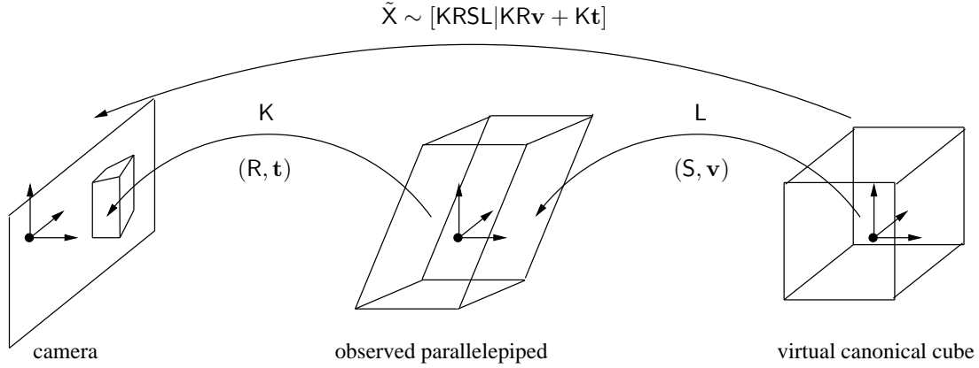
Figure 3.1: The projection of the canonic parallelepiped (cube) into the image. Matrices K , L correspond to intrinsic parameters of camera and parallelepiped and (R, \mathbf{t}) , (S, \mathbf{v}) correspond to extrinsic parameters of camera and parallelepiped, respectively.
