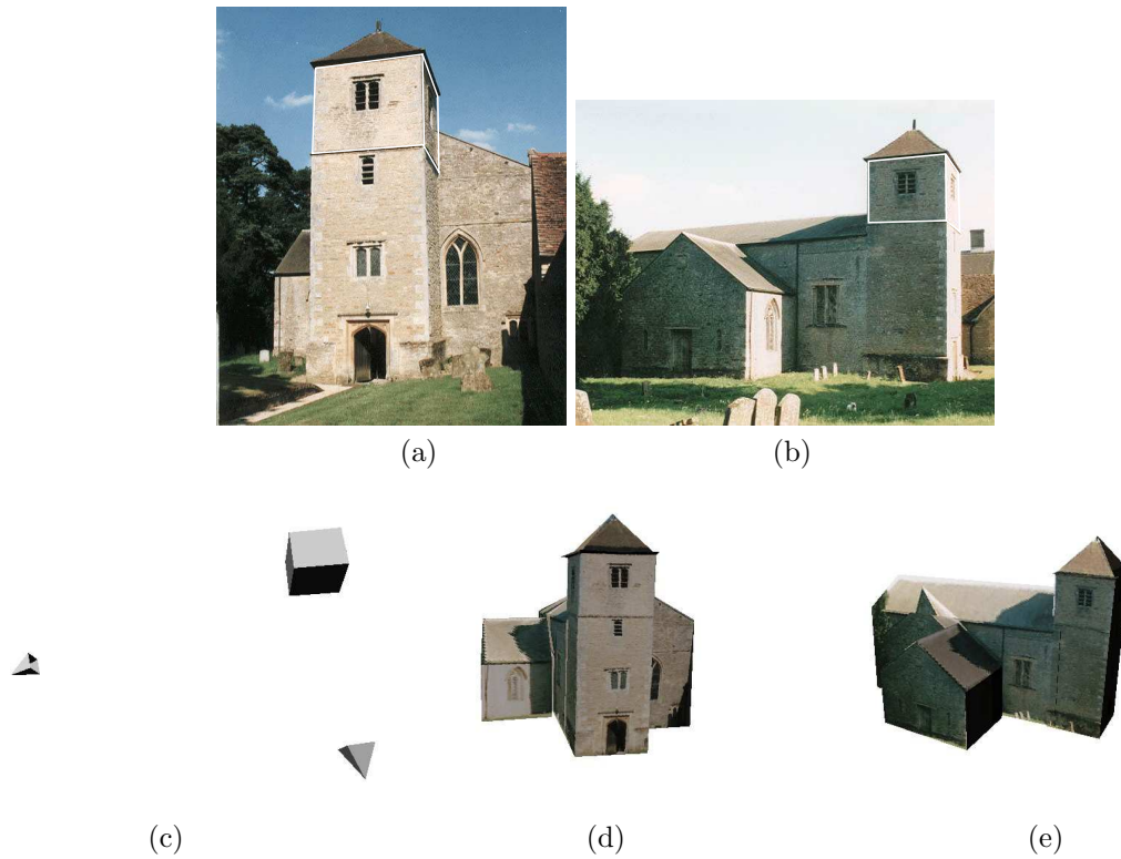
Figure 7.17: Chetwode church: (a),(b) The original images (courtesy of Mr. Kevin Quick); (c) Reconstructed calibration primitive and cameras; (d),(e) Screen-shots of the reconstructed model.
