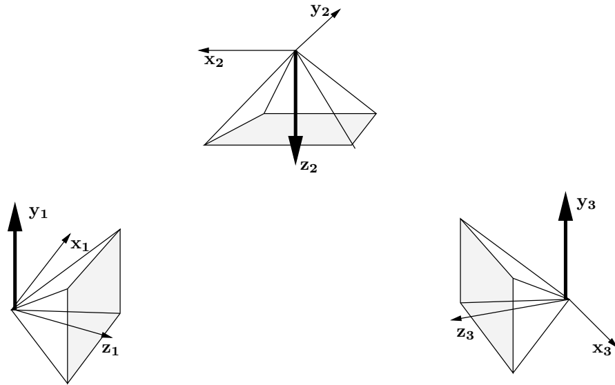
Figure 4.3: Illustration of critical motion for cameras of type C (only principal point is known): one axis per camera (axes y_1 , z_2 and y_3 ) is pointing in some common direction.
