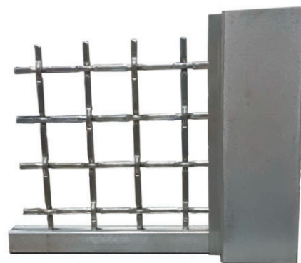
Wire Mesh Framed out with 1" MP-1A and inserted into 3" Universal Enclosure Post
