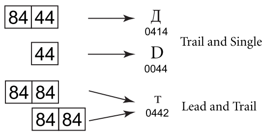
Figure 2-9. Overlap in Legacy Mixed-Width Encodings
